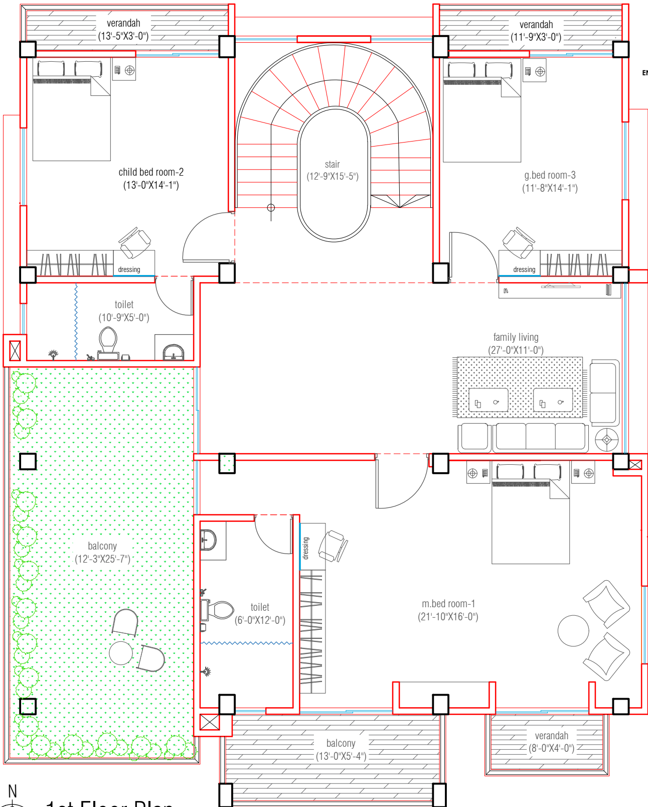
1st Floor Plan (10'-0" Slab to Slab)
